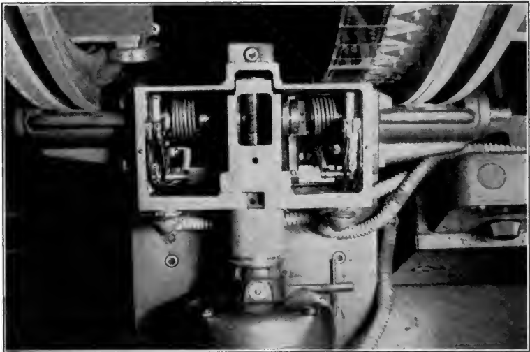
FIG. 4. Close-up of spring element and overrunning clutch, which assures accurate, rapid indexing of the drums.
